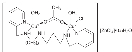
Fig. 2 Molecular structure proposed for the copper(II) compound 1
